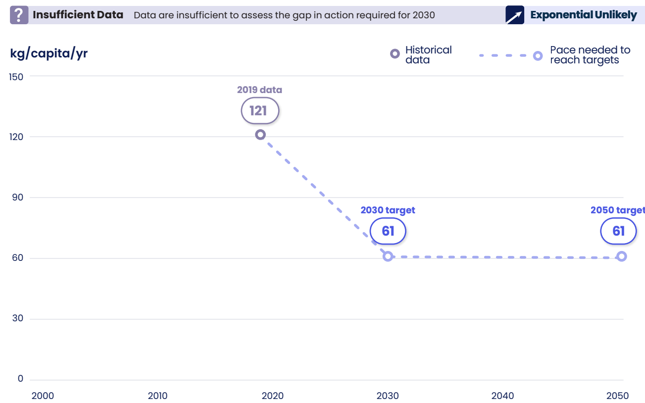
FIGURE 65 | Historical progress toward 2030 and 2050 targets for food waste
