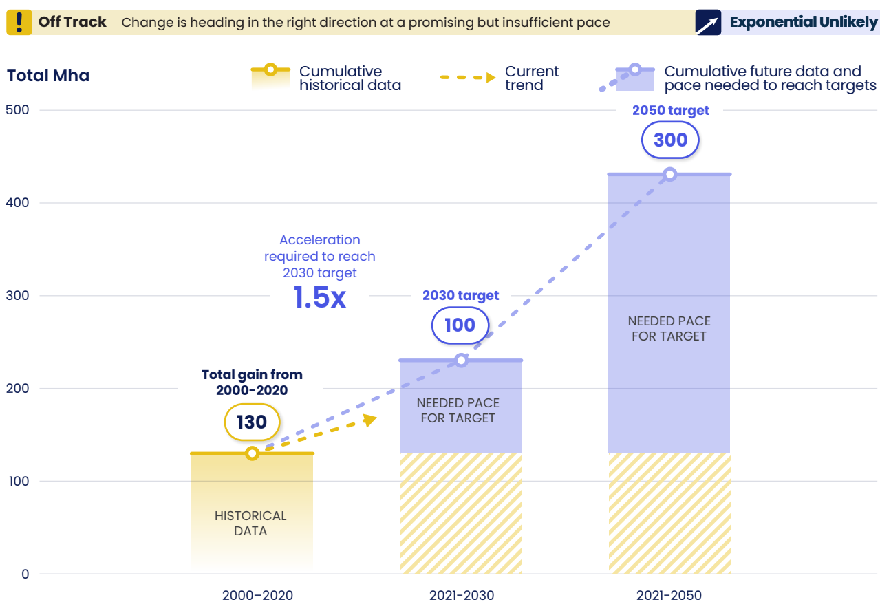
FIGURE 46 | Historical progress toward 2030 and 2050 targets for reforestation
